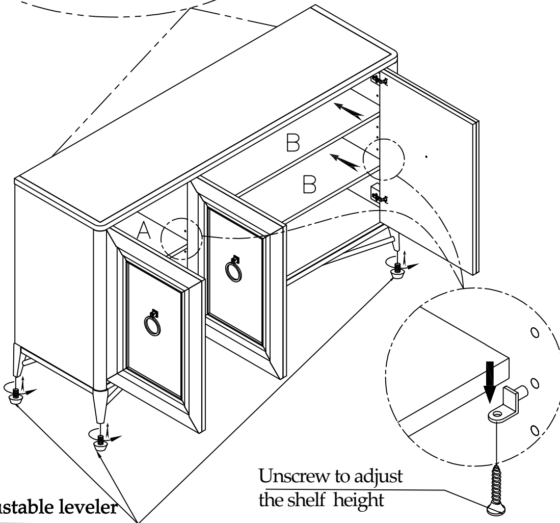
Furniture Tipping Restraint Kit (A) (Inside White Plastic Bag)
