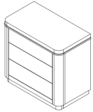
21869 3-Drawer Nightstand
